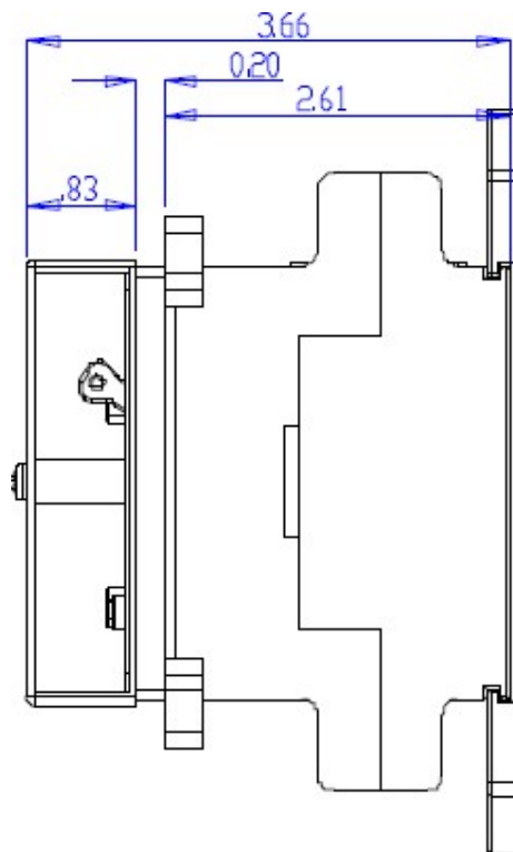
Suggested mounting for Panel Mount GFP Relay
