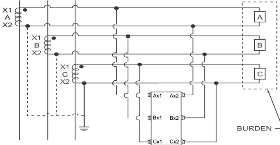
TYPICAL 3 ELEMENT CONNECTION DIAGRAM 3-OCP-XXX
